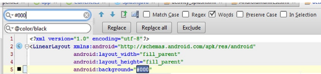
Figure 9-11. Replacing hard-coded color values with named references in the colors.xml file
