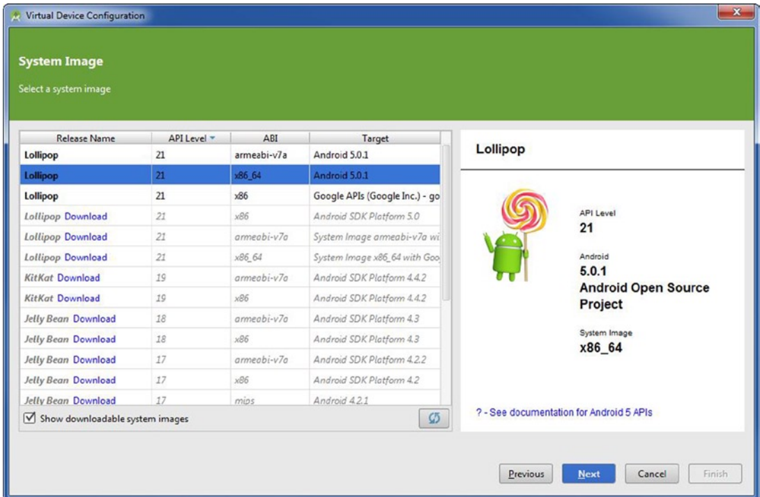
Figure 1-27. Select the x86_64 system image
