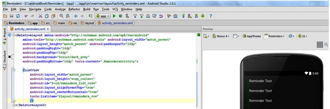
Figure 5-16. The preview pane is now rendering a custom ListView layout
