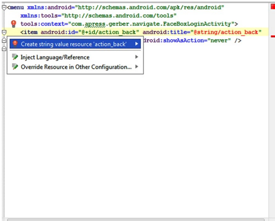
Figure 14-20. Editing the FaceBox menu
