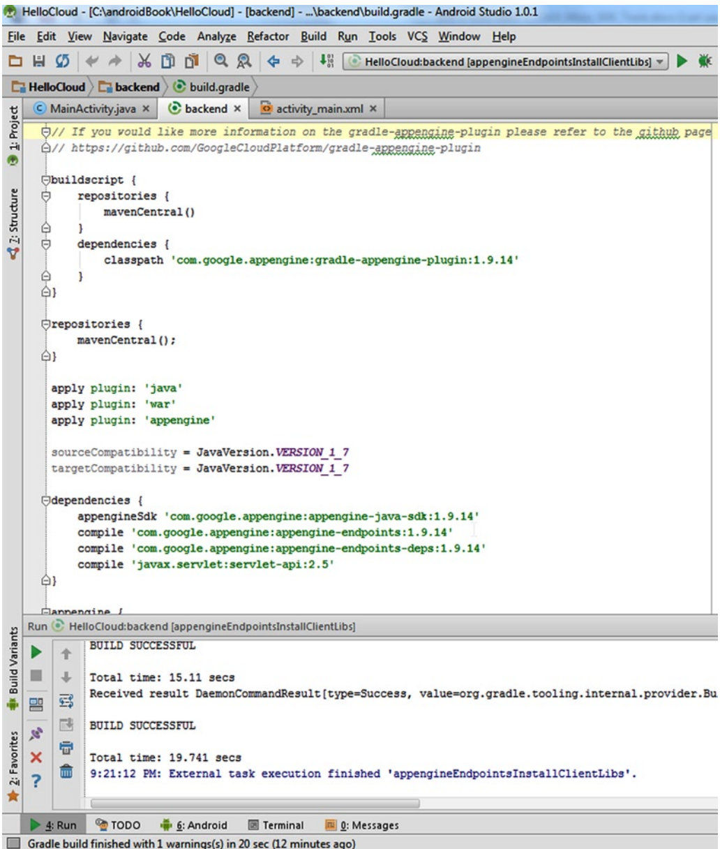
Figure 14-25. Install the client libs for your endpoint
