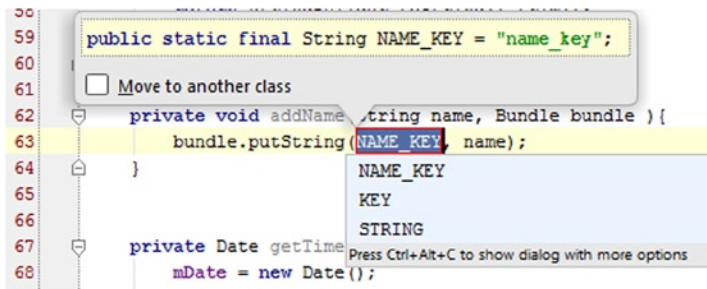
Figure 4-9. Extract Constant NAME_KEY
