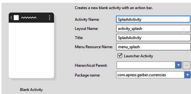
Figure 9-18. New ► Activity ► Blank Activity to create SplashActivity
