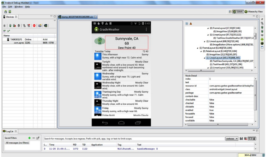
Figure 14-6. Exploring the Gradle Weather UI by using a hierarchy ump
