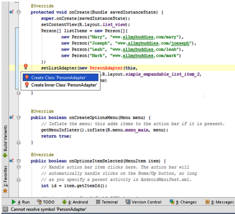
Figure 8-19. Add PersonAdapter inside onCreate() method
