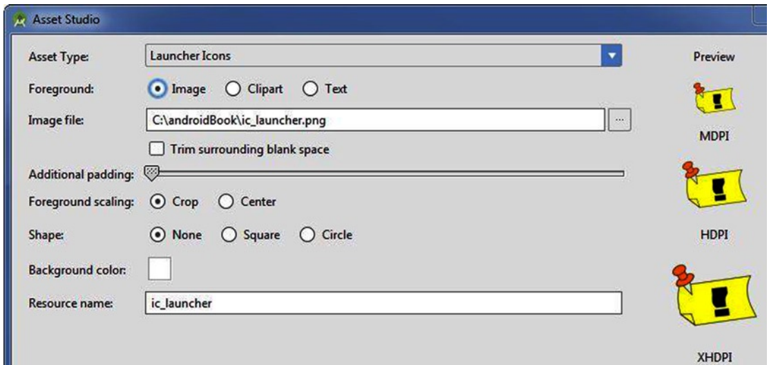
Figure 6-12. New Image Asset dialog box
