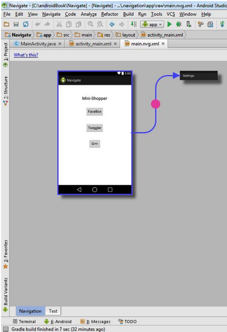
Figure 14-16. Opening the Navigation Editor
