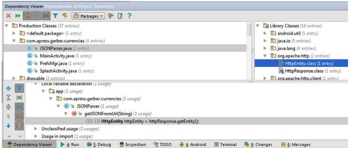
Figure 11-15. Analyze Dependencies tool window showing dependency on org.apache.http.HttpEntity.class
