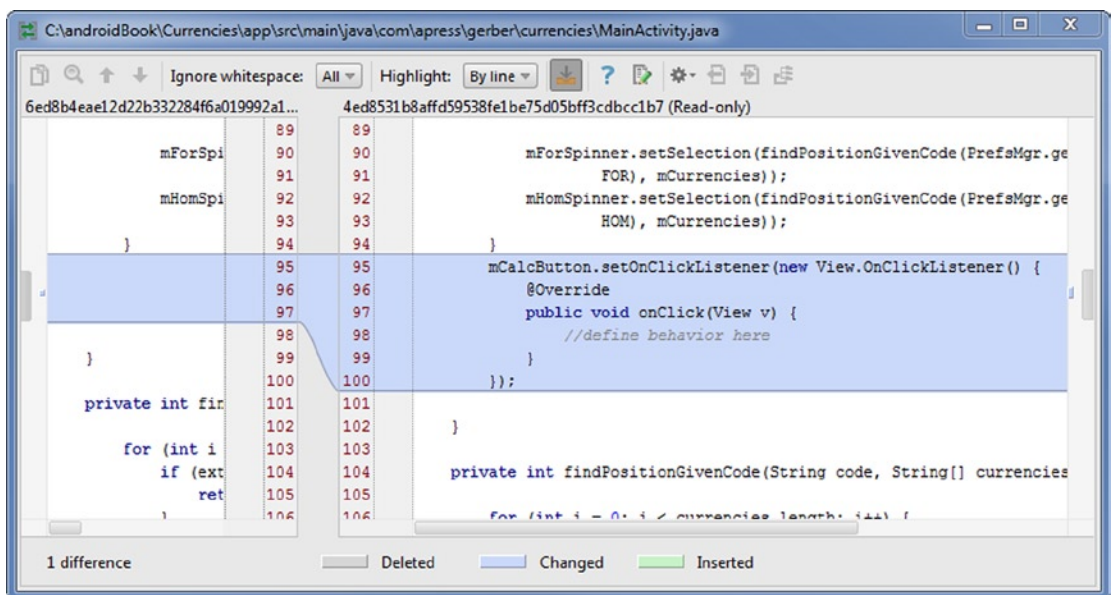
Figure 10-19. Create an anonymous inner class to handle button click behavior
