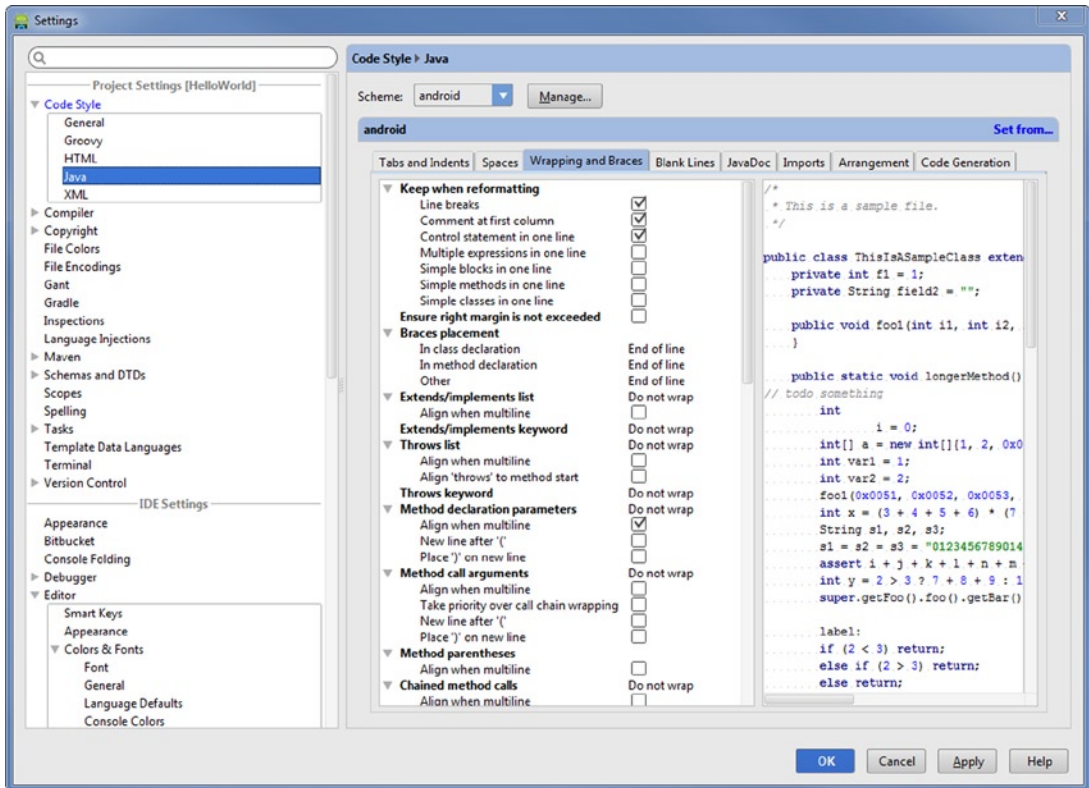
Figure 3-21. Settings dialog box with Code Style > Java selected and showing the Wrapping and Braces tab
