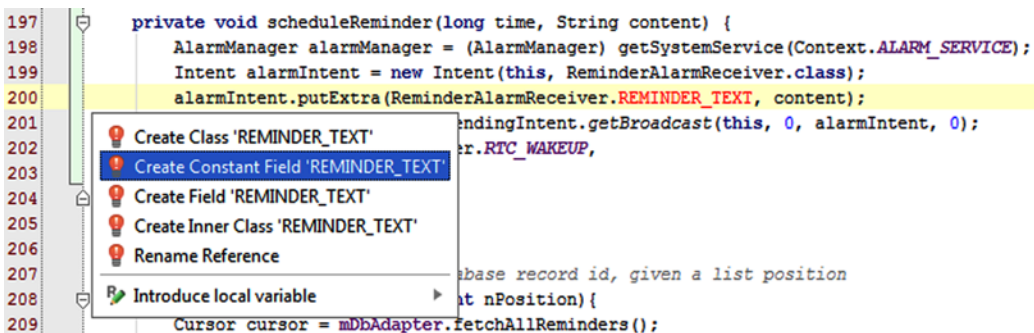
Figure 7-18. Generate a Constant field
