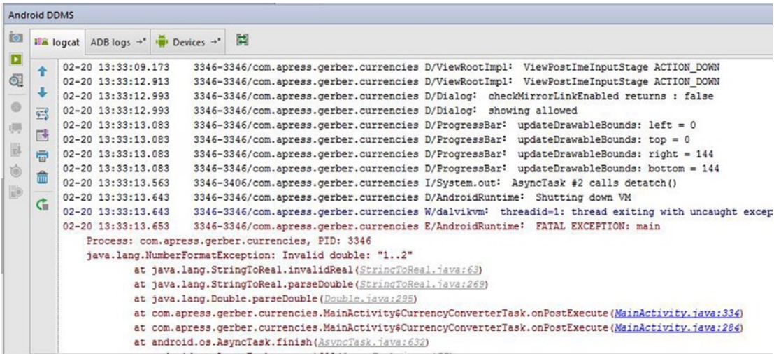
Figure 11-16. Logcat window with verbose logs and stack trace
