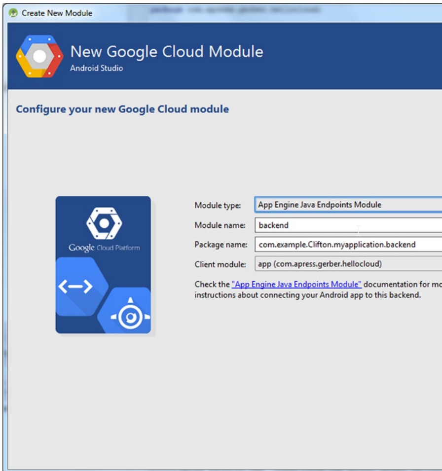
Figure 14-23. Select App Engine Java Endpoints Module
