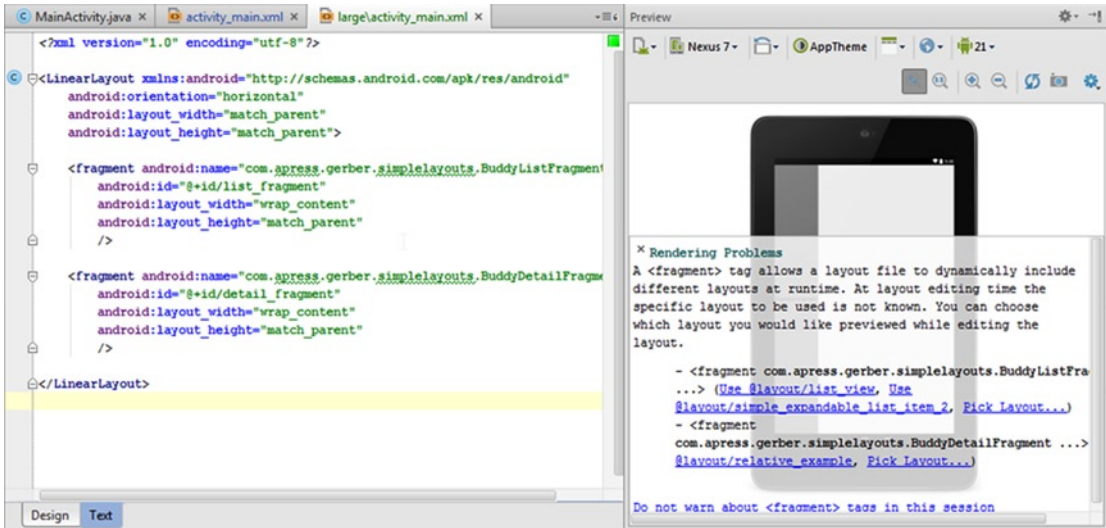
Figure 8-29. Linear layout containing fragments
