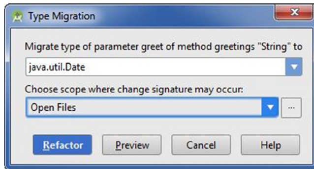
Figure 4-4. Type migration from string to date
