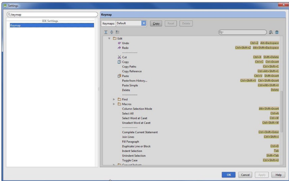
Figure 16-9. From Settings ► Keymap, double-click entries to modify or create keyboard shortcuts
