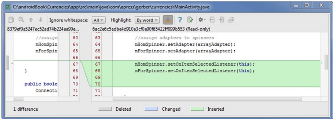
Figure 10-6. Delegate the behavior of spinners to MainActivity
